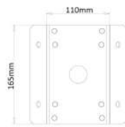
External Corner Bracket
